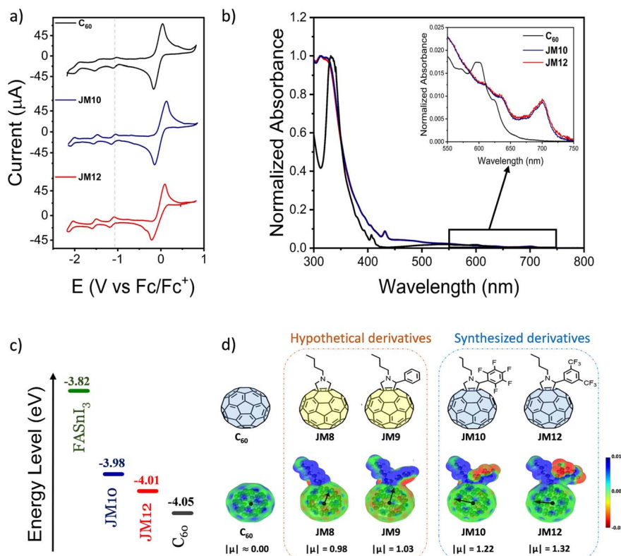
Fig. 1 (a) CV of C_{60} , JM10 , and JM12 in acetonitrile : o -dichlorobenzene (1 : 4) ( NB_4^+PF_6^- 0.1 M was employed as supporting electrolyte) vs. Fc/Fc + couple, dotted line is an eye guide. (b) UV-vis absorption spectra of the fullerene derivatives in chlorobenzene ( 1 \times 10^{-5} M). (c) Schematic illustration of the LUMO levels for the different fullerene derivatives, extracted from (a) and conduction band of FASnI 3 perovskite, extracted from ref. 45. (d) Molecular electrostatic potential at \rho = 0.001 a.u. Range of values of the electrostatic potential: from -0.01 (red) to 0.01 (blue). Black arrows indicate the net dipole moment direction.
